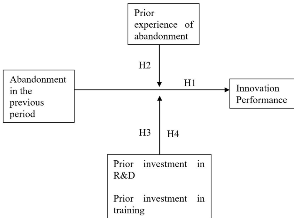
Figure 1: Theoretical model
